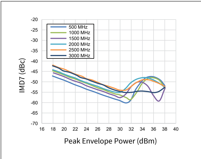
Figure 18. IMD7 vs. Peak Envelop Power as a Function of Frequency
