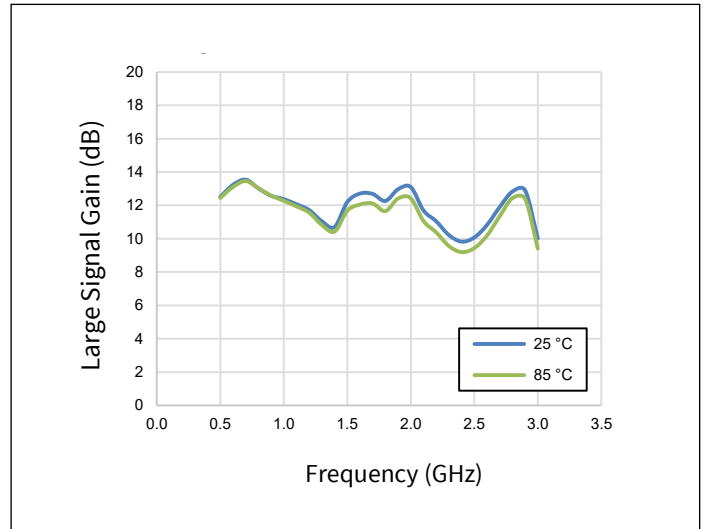
Figure 13. Large Signal Gain vs. Frequency as a Function of Temperature
