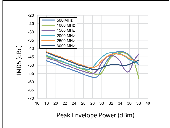
Figure 17. IMD5 vs. Peak Envelop Power as a Function of Frequency
