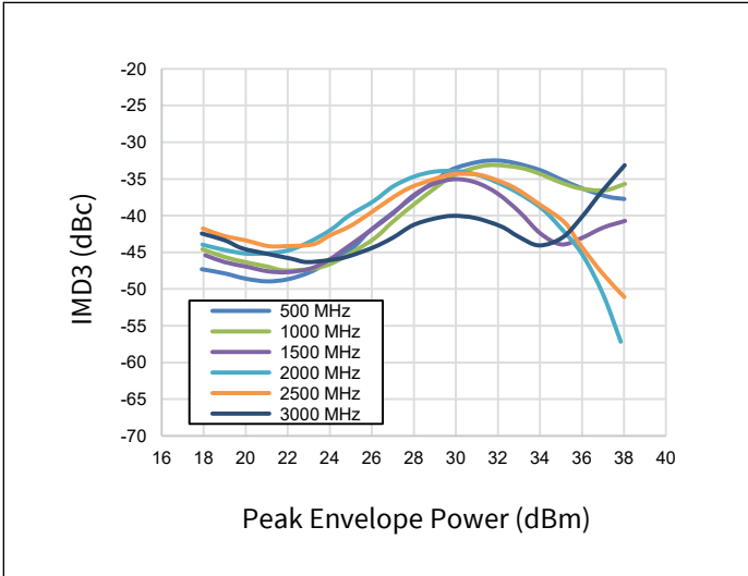
Figure 16. IMD3 vs. Peak Envelop Power as a Function of Frequency
