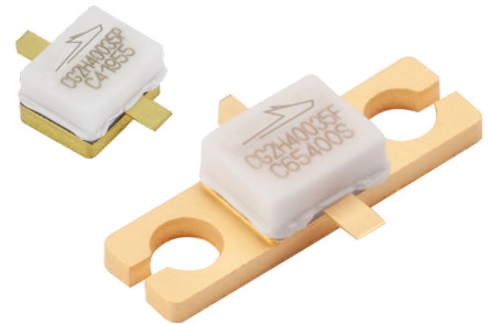
Package Types: 440196 & 440166 PNs: CG2H40035P & CG2H40035F
