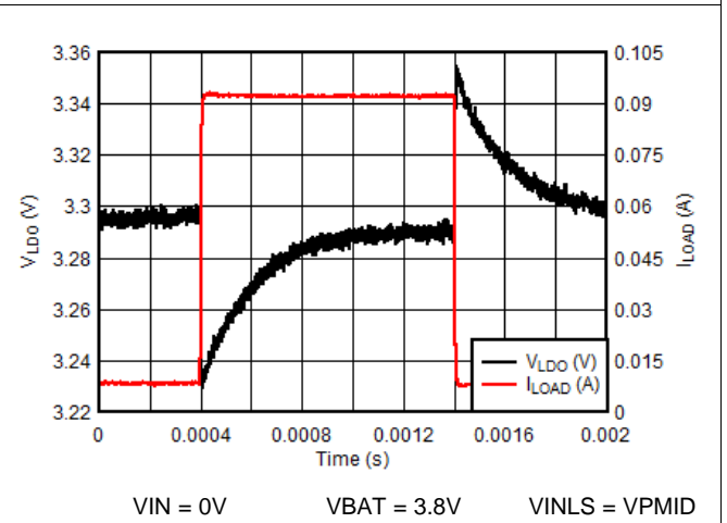
Figure 102. LDO Load Transient - VLDO = 3.3V
