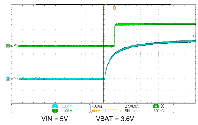
Figure 95. \overline{\text{PG}} \overline{\text{MR}} Level Shift Function - \overline{\text{MR}} Rising
