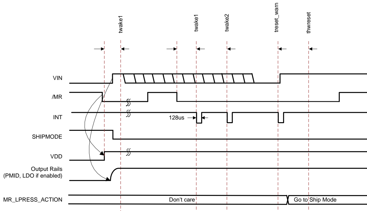
Figure 19. MR Wake from Ship Mode – V_{\text{IN}} Dependencies
