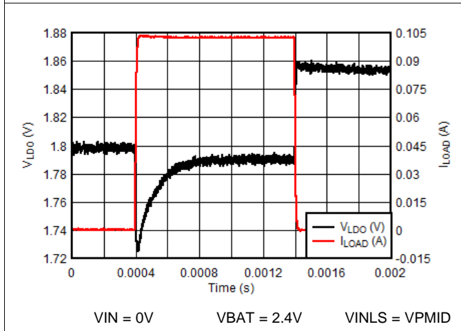
Figure 101. LDO Load Transient - VLDO = 1.8V
