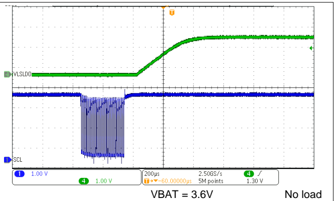
Figure 98. LDO Enable Through I 2 C (EN_LS_LDO)
