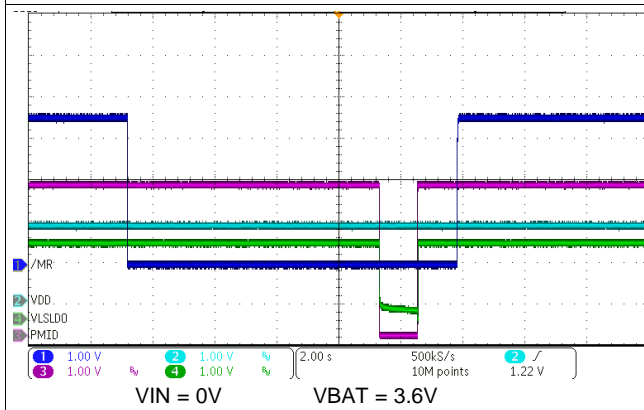
Figure 89. HW Reset on \overline{MR} Long Button Press
