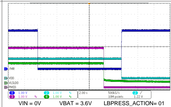
Figure 90. Ship Mode Entry with \overline{MR} Long Button Press
