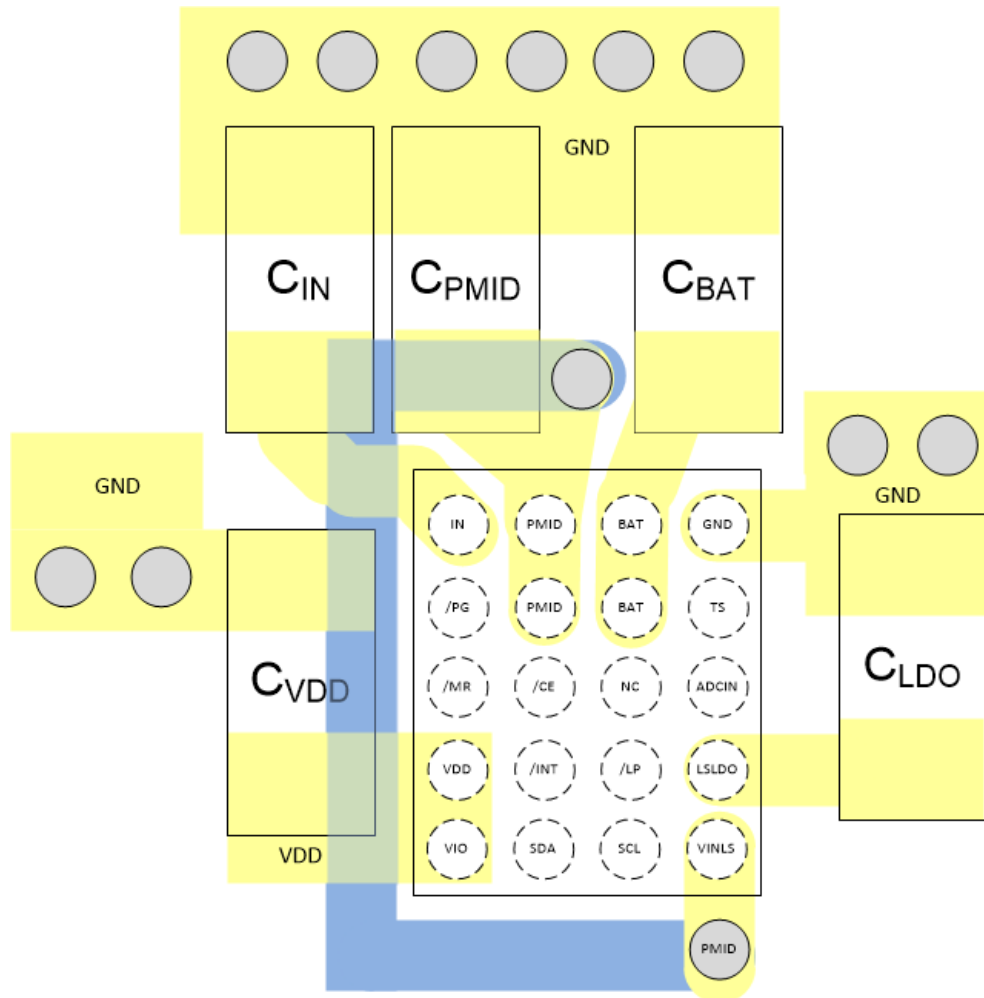
Figure 104. Layout Example
