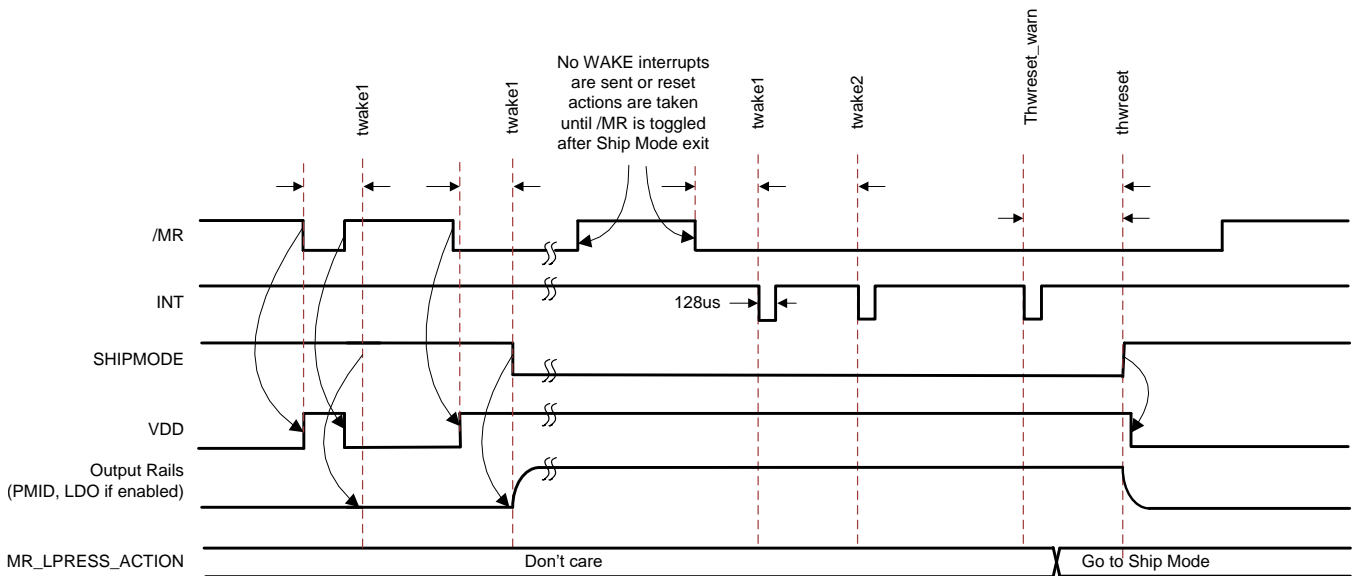
Figure 18. MR Wake from Ship Mode ( \text{MR\_LPRESS\_ACTION} = \text{Ship Mode} , V_{\text{IN}} not valid)
