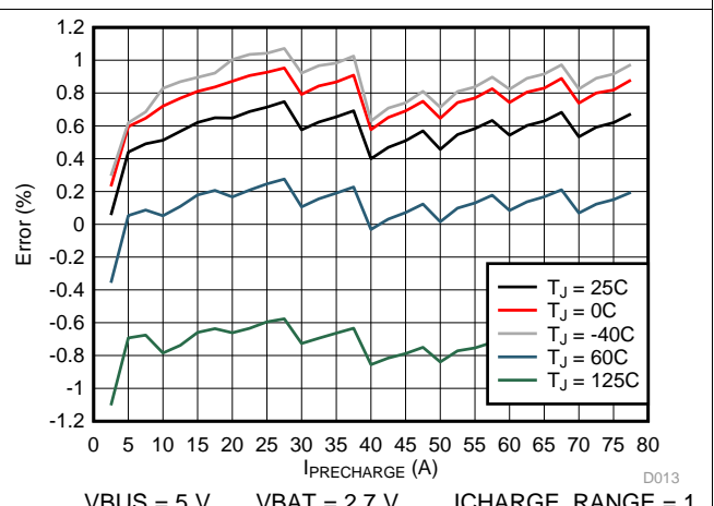
Figure 4. Pre-Charge Current Accuracy vs. IPRECHARGE Setting (ICHARGE_RANGE = 1)
