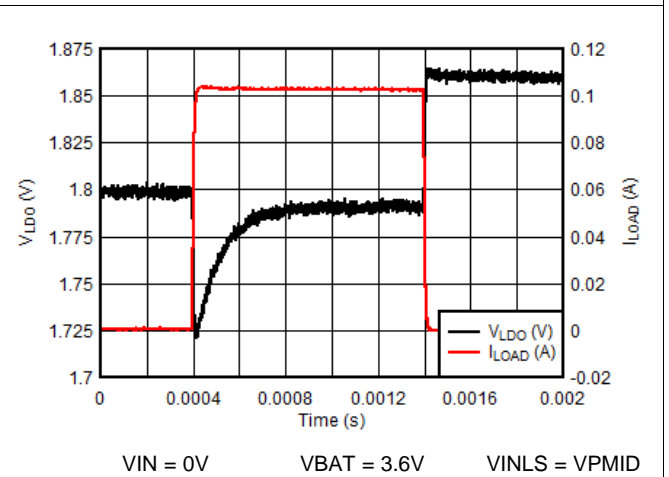
Figure 100. LDO Load Transient - VLDO = 1.8V
