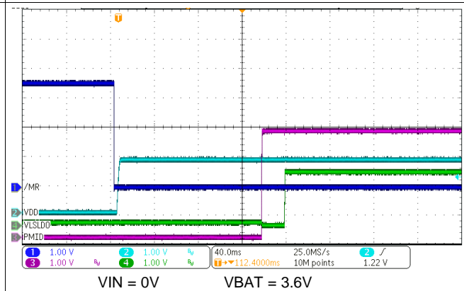
Figure 88. Power Up from Ship Mode with \overline{MR} Press
