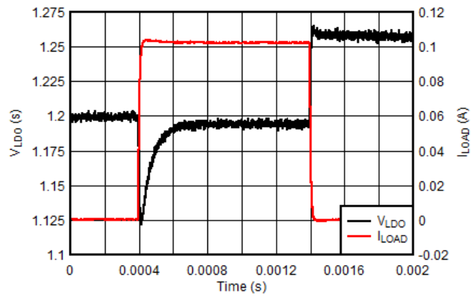
Figure 103. LDO Load Transient - VLDO = 1.2V
