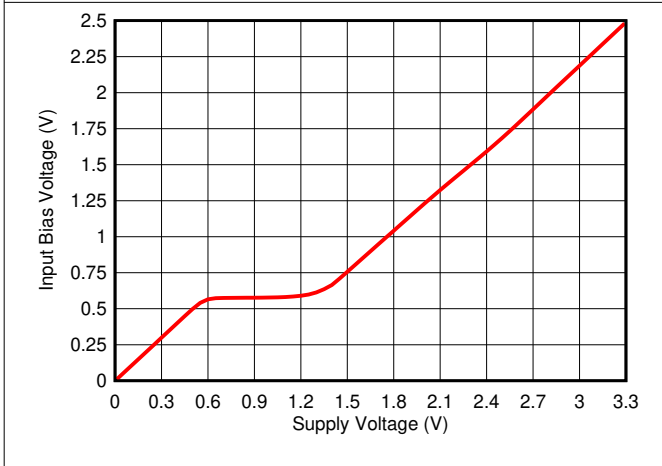
Figure 6-35. Input Bias Voltage vs Supply Voltage
