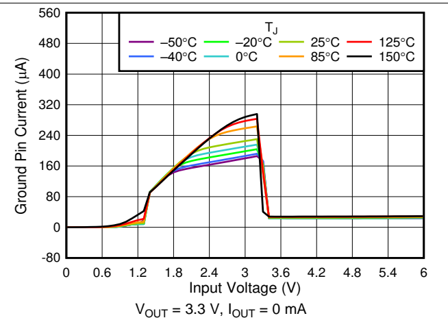
Figure 10. I_{GND} vs V_{IN}
