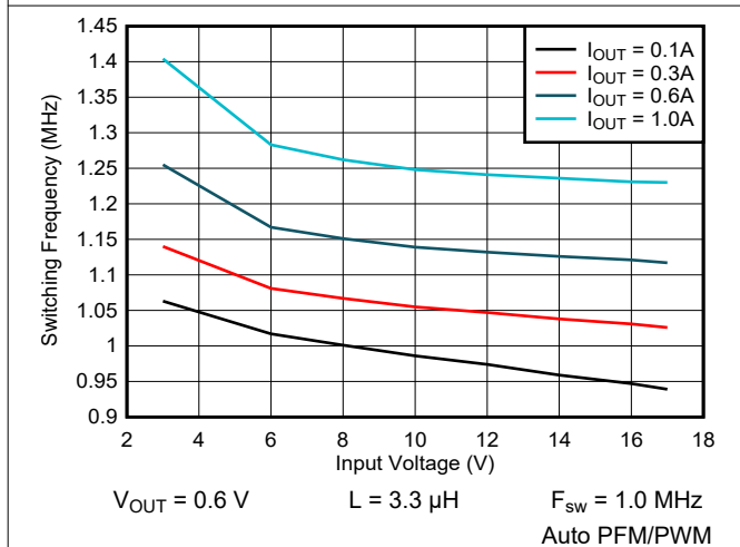
Figure 9-58. Switching Frequency vs Input Voltage
